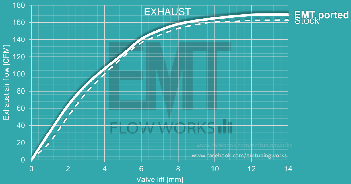
BMW M4 S55 stage1+ Ported head stage1+ stock valves
