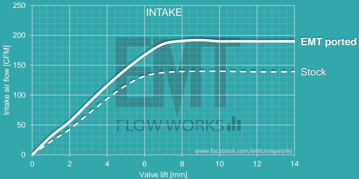
BMW M4 S55 stage1+ Ported head stage1+ stock valves
